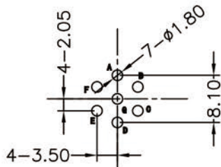
PCB SCALE
