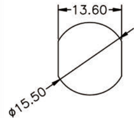
RECOMMENDED PANEL CUTOUT SIZE
