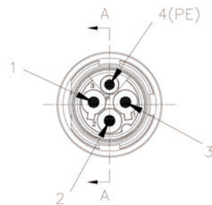
LEFT VIEW
