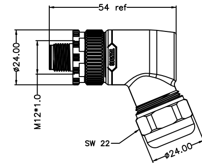
TERMINAL:SCREW
